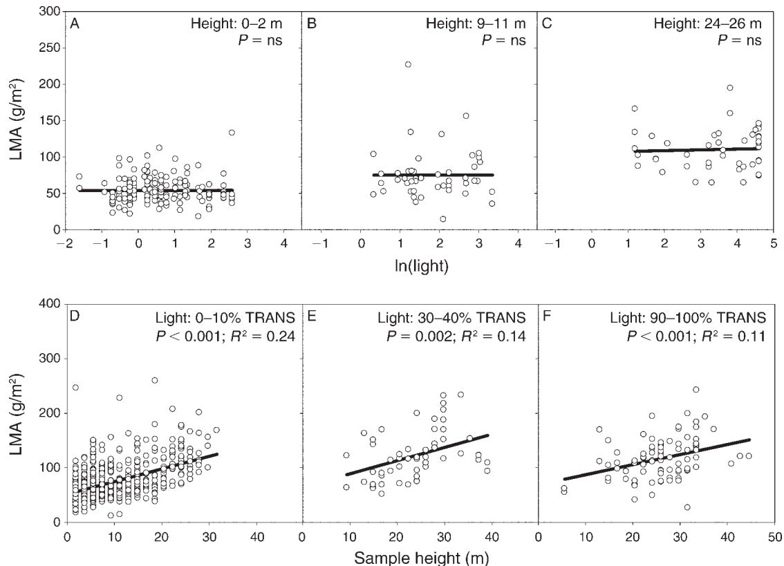
FIG. 5. For all functional groups pooled, LMA is plotted against ln(light) for three narrow bands of height (panels A-C), and against height for three narrow bands of light (panels D-F). Figures show no change in LMA with light at three height levels, but significant increase in LMA with height at three light levels. The abbreviation "ns" indicates not significant.
