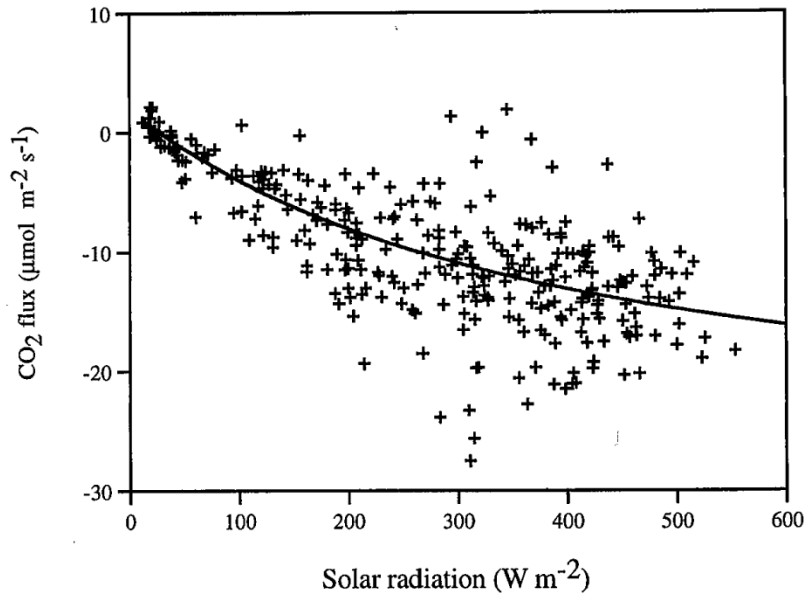
FIGURE 1. Relationship between net ecosystem exchange measured by eddy covariance and solar radiation. The solid line is nonlinear fit of simple photosynthesis model (Equation 2, r^2 = 0.36 ). NEE values include points with frictional velocity ( u^* ) > 0.2 \text{ m s}^{-1} .
