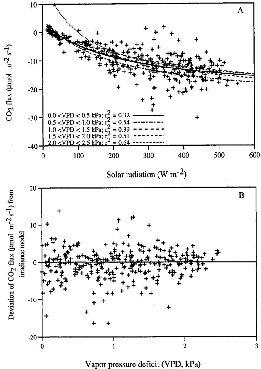
FIGURE 2. (A) Relationship between net ecosystem exchange measured by eddy covariance and solar radiation at different vapor pressure deficits (VPD). Lines are nonlinear fits of simple photosynthesis model (Equation 2) for data in ranges of VPD. Values of r^2 are from logarithmic fits to data. Values only include points with frictional velocity ( u^* ) > 0.2 m s -1 . (B) Relationship between deviation of measured eddy flux from solar radiation model (FIGURE 1) and vapor pressure deficit. Solid line indicates zero line.
