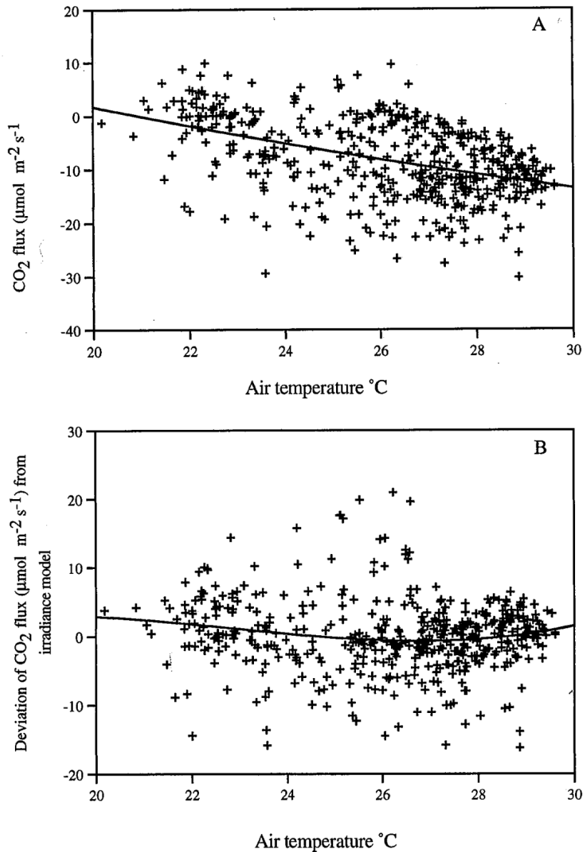
FIGURE 3. (A) Relationship between net ecosystem exchange measured by eddy covariance and air temperature. The solid line represents logarithmic fit to the data ( r^2 = 0.20 ). (B) Relationship between deviation of measured eddy flux from solar radiation model (FIGURE 1) and air temperature. Solid line represents 2nd order polynomial fit to the data.
