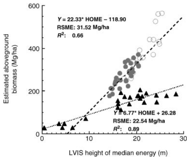
Fig. 3 Simple linear regression analysis for lidar height of median energy (m) vs. plot-level allometrically estimated above-ground biomass (Mg/ha) for TMF (circles, dashed line, upper left equation) and TWF (triangles, dotted line, lower left equation) study areas. The open circles in the TMF regression relationship indicate plots that contain stems whose diameters are larger than the original distribution sampled to develop the allometric equation (eqn 2) and were not included in the regression analysis. R^2 values are coefficients of determination from regression analysis.
