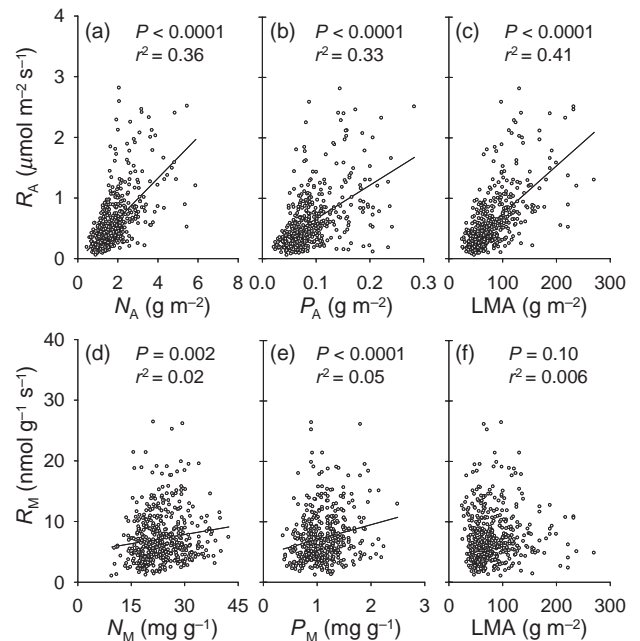
Figure 2. Regression plots between area- (plots a–c) and mass-based (plots d–f) foliar respiration, nitrogen, phosphorus and leaf mass per area (LMA). Leaf-area-based correlations between respiration and foliar nutrients (plots a & b) were stronger than mass-based correlations (plots d & e). Equations for each significant ( P < 0.05 ) regression were: R_A = -0.03 + 0.34 \times N_A ; R_A = 0.04 + 6.5 \times P_A ; R_A = -0.05 + 0.008 \times \text{LMA} ; R_M = 4.77 + 0.10 \times N_M ; and R_M = 4.3 + 2.5 \times P_M .
