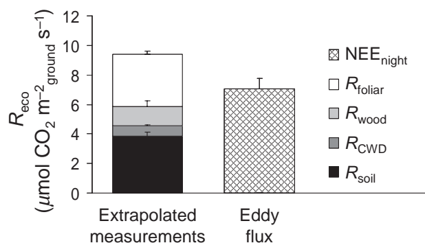
Figure 5. A comparison of ecosystem respiration ( R_{\text{eco}} ), as estimated by eddy flux night-time net ecosystem exchange ( NEE_{\text{night}} ) versus the summation of extrapolated measurements of component parts. R_{\text{eco}} from extrapolated measurements ( 9.40 \pm 0.47 \mu\text{mol CO}_2 \text{ m}^{-2} \text{ s}^{-1} ) was 33% higher than NEE_{\text{night}} ( 7.05 \pm 0.69 \mu\text{mol CO}_2 \text{ m}^{-2} \text{ s}^{-1} ; Loescher et al. 2003) for the same forest. NEE_{\text{night}} was based on data for turbulent nights only, when friction velocity ( u^* ) was greater than 0.4 \text{ m s}^{-1} (Loescher et al. 2003). For the old-growth forest at La Selva, soil respiration was 3.88 \pm 0.22 \mu\text{mol CO}_2 \text{ m}^{-2} \text{ s}^{-1} (Schwendenmann et al. 2003); woody respiration was 1.34 \pm 0.36 \mu\text{mol CO}_2 \text{ m}^{-2} \text{ s}^{-1} (Cavaleri et al. 2006); coarse woody debris (CWD) respiration was estimated to be 0.66 \pm 0.05 \mu\text{mol CO}_2 \text{ m}^{-2} \text{ s}^{-1} , from published total CWD carbon and turnover time (Clark et al. 2002); and foliage respiration was 3.5 \pm 0.2 \mu\text{mol CO}_2 \text{ m}^{-2} \text{ s}^{-1} using estimate (1) of this study (Table 2).
